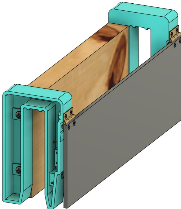
Target assembly (without light)
