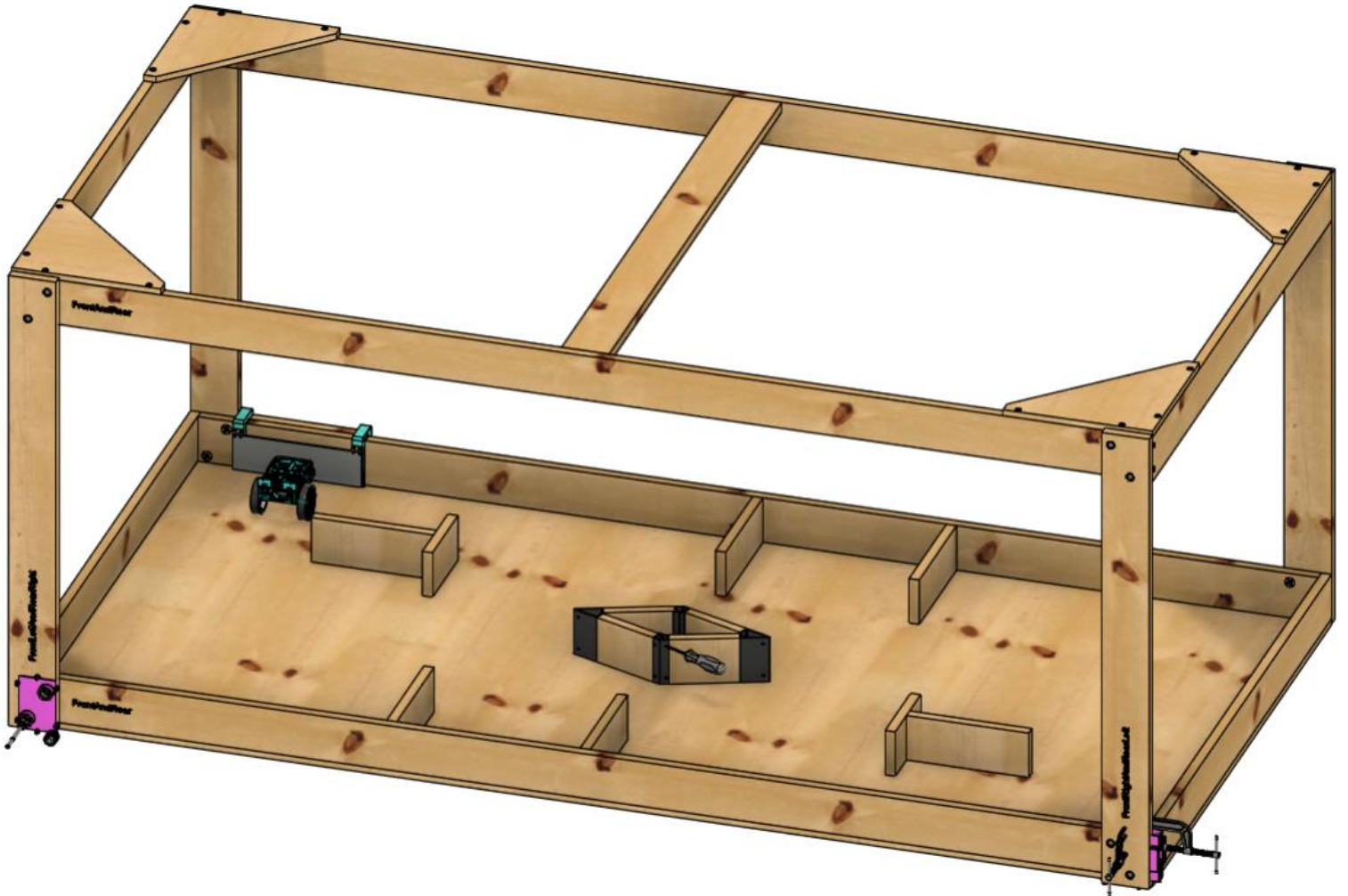
Base after painting
